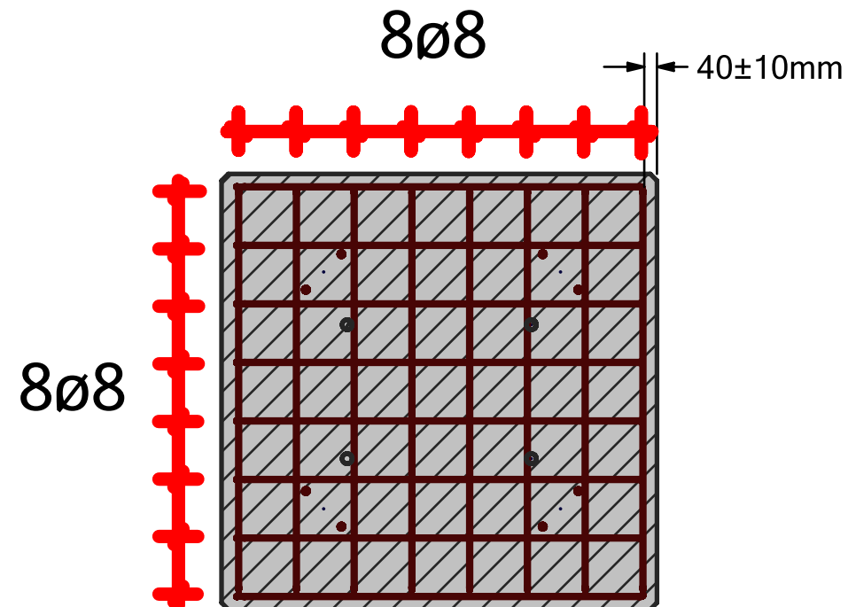
SECTION B-B
